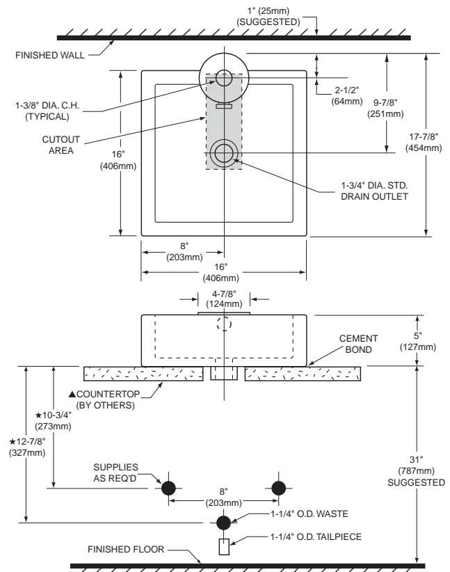
Shown with Iperbole faucet (5131.101.002)
