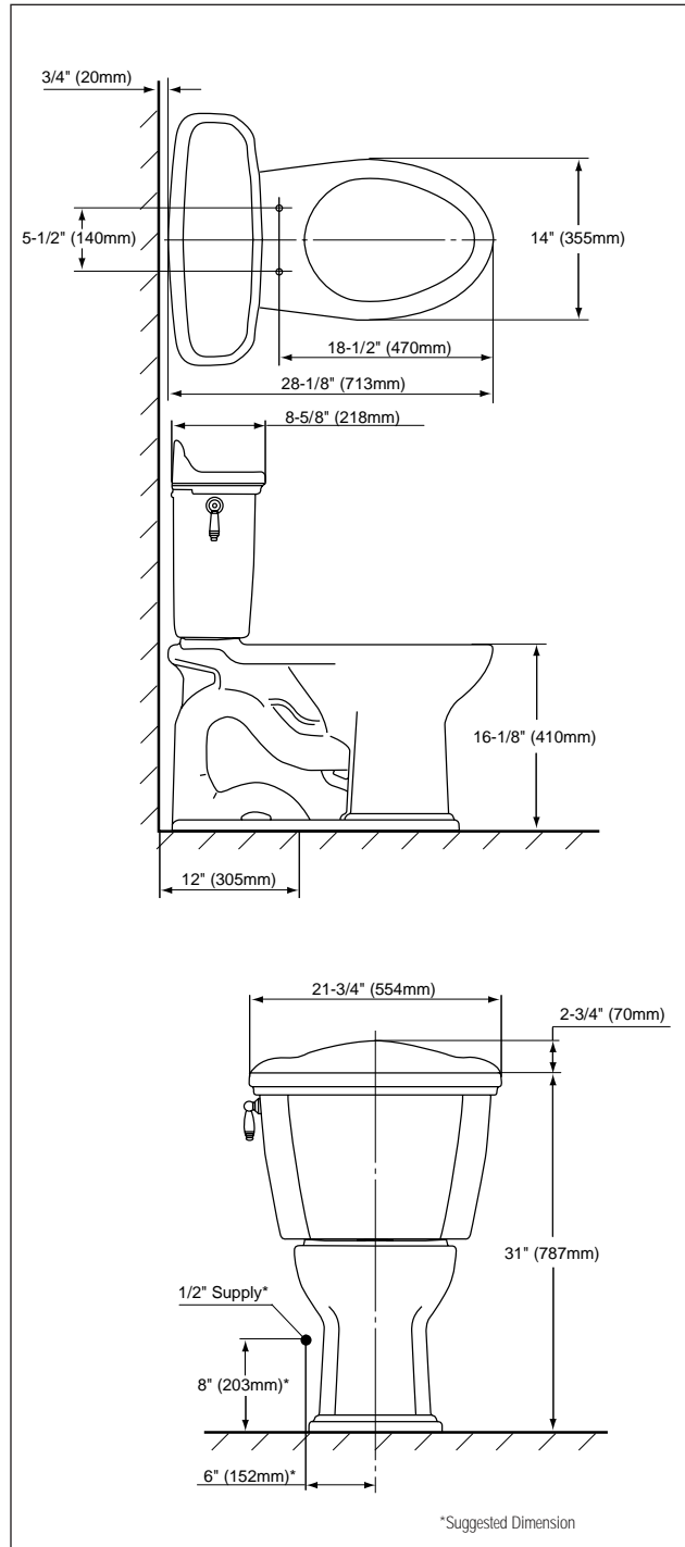
CST754SFN - Whitney™ Toilet
